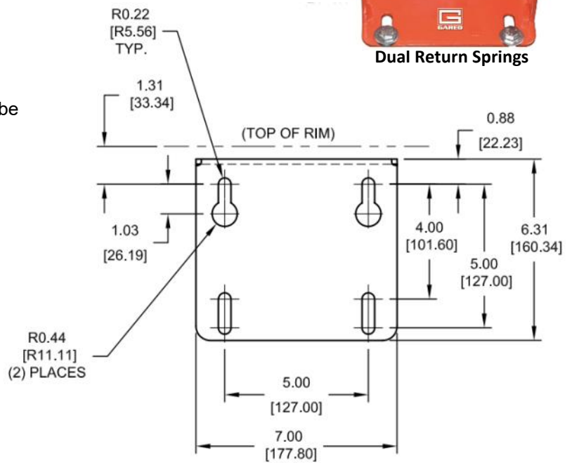
MOUNTING PLATE VIEW
